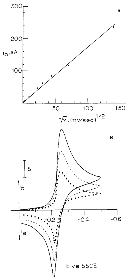
Figure 2. (A) i_p vs. v^{1/2} for the cathodic branch of the first reduction of poly(benzyl viologen) on Pt in DMF/0.1 M TBAP solution. (B) Cyclic voltammograms on Pt for poly(benzyl viologen) in DMF/0.1 M TBAP at different sweep rates. Solid curve = 200, dashed curve = 50, dotted curve = 20 mV/s. S = 5 \mu\text{A} .
