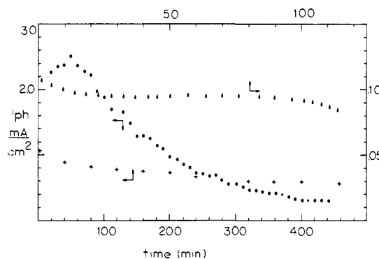
Figure 4. Long-term operation of surface-modified p-Si electrodes for \text{H}_2 evolution. Conditions: thoroughly degassed aqueous 0.2 M NaTFA, pH 2.1, 0.2 M \text{LiClO}_4 . Illumination by 450-W Xe lamp with 590-nm cutoff filter (intensity ca. 110 \text{mW}/\text{cm}^2 ). Applied bias: (▲) -0.1 V, (●) -0.175 V, (+) -0.1 V.
