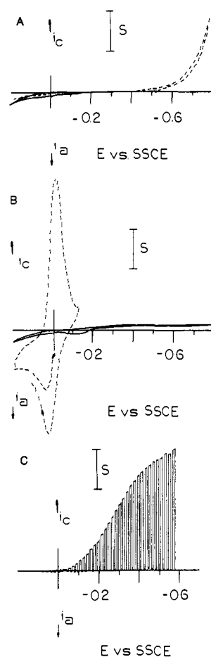
Figure 3. Electrochemical response in the dark (solid curve) and under illumination (dashed curve) for (A) bare p-Si, S = 5 \mu\text{A} ; (B) p-Si/poly(benzyl viologen), S = 5 \mu\text{A} ; (C) p-Si/poly(benzyl viologen)/ \text{Pt}^0 under chopped illumination, S = 100 \mu\text{A} . Conditions: deaerated aqueous solution 0.2 M sodium trifluoroacetate, pH 2.1, 0.2 M \text{LiClO}_4 . Sweep rate = 50 mV/s except for part C (10 mV/s). Illumination using a 450-W Xe lamp with a 590-nm cutoff filter (input power density ca. 100 \text{mW}/\text{cm}^2 ).
