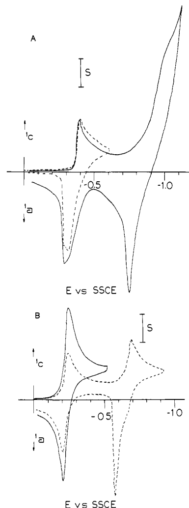
Figure 1. (A) Cyclic voltammogram on Pt of poly(benzyl viologen) (1 mg/mL) in aqueous (pH 9.0) 0.1 M KBr solution. Sweep rate = 100 mV/s. Dashed curve = scan reversal after first wave. S = 20 \mu A . (B) Cyclic voltammogram on Pt of poly(benzyl viologen) (1 mg/mL) in DMF/0.1 M TBAP solution. Sweep rate = 100 mV/s. Solid curve = scan reversal after first wave. Solid curve: S = 5 \mu A , dashed curve: S = 10 \mu A .
